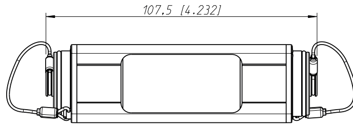
NO2-4FDW-A opticalCON DUO
