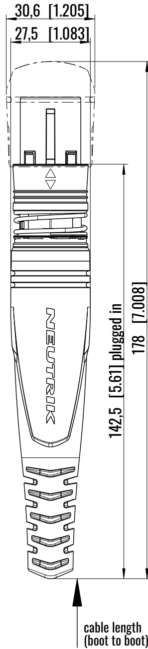
opticalCON DUO SMPTE
