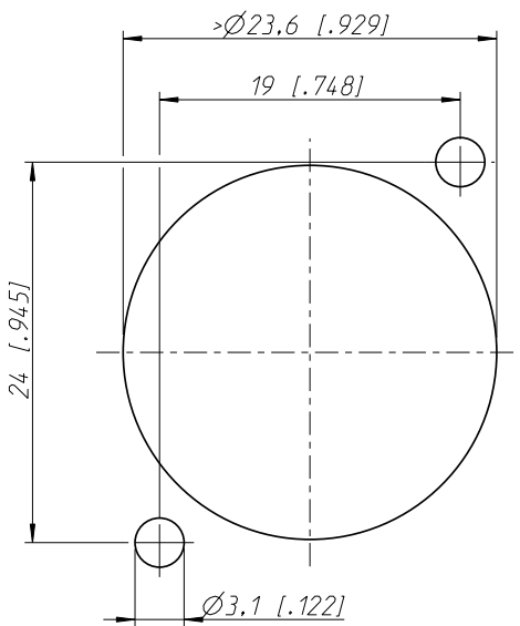
panel cut out (rear side)
