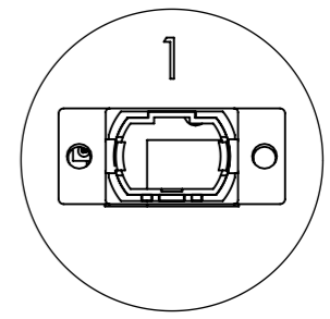
DETAIL B MTP-MPO X 4 SCALE 2 : 1.6
